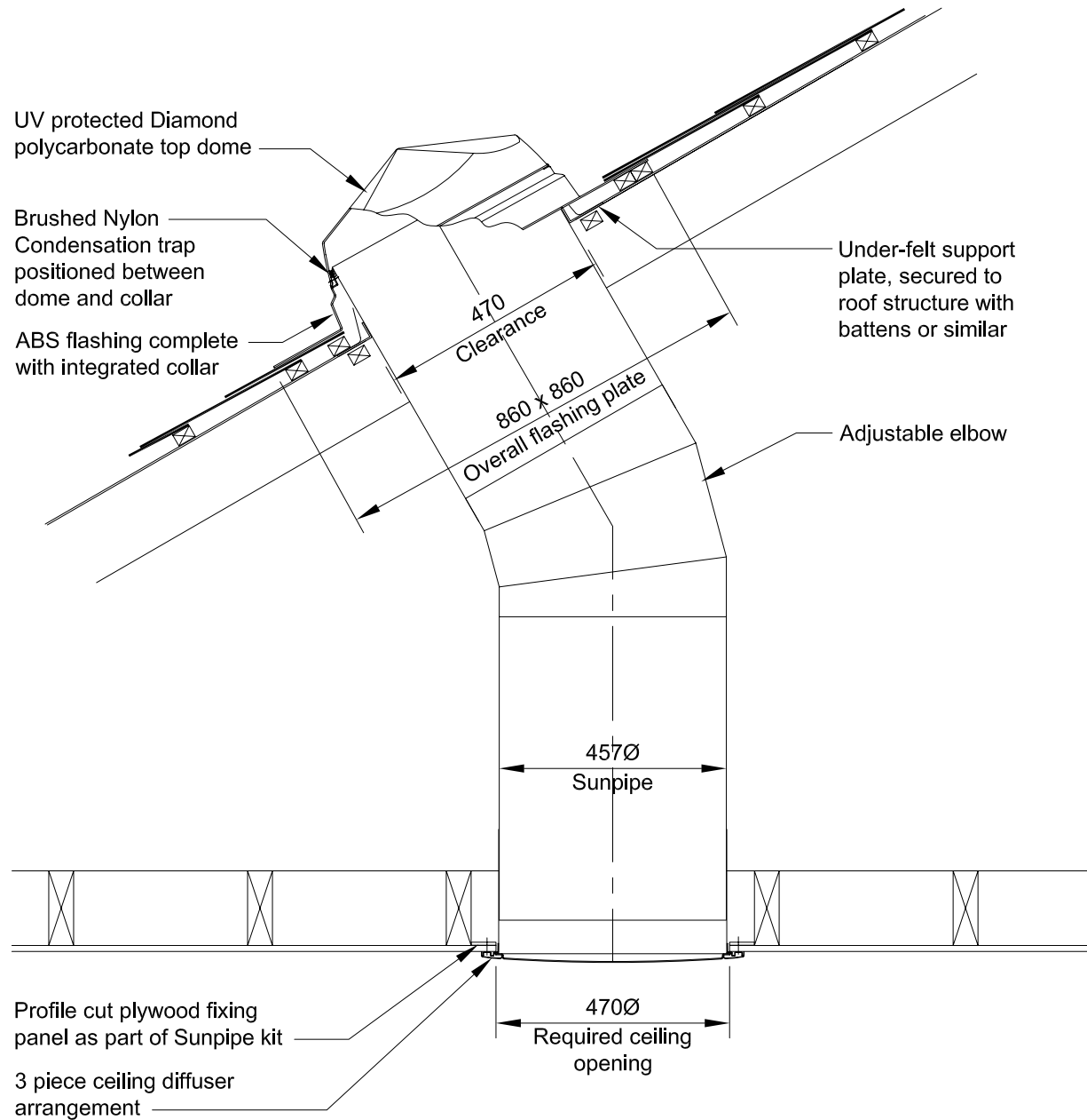
Section
