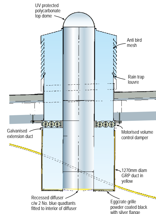
Plan of Damper arrangement
