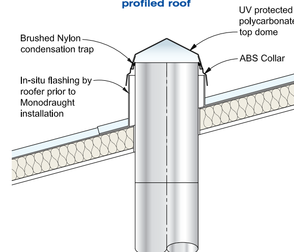
SunPipe flashing detail to metal profiled roof
