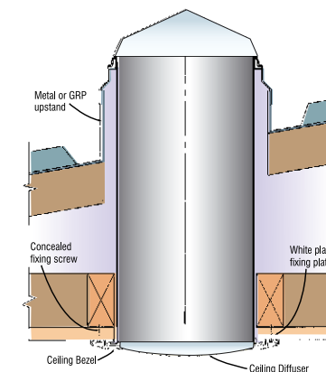
Alternative GRP upstand for British Steel type colour coated roofing sheet, bonded to surface
