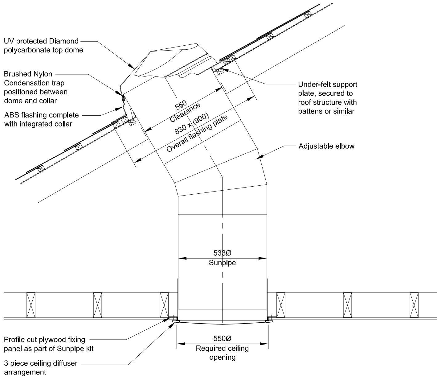
Section
